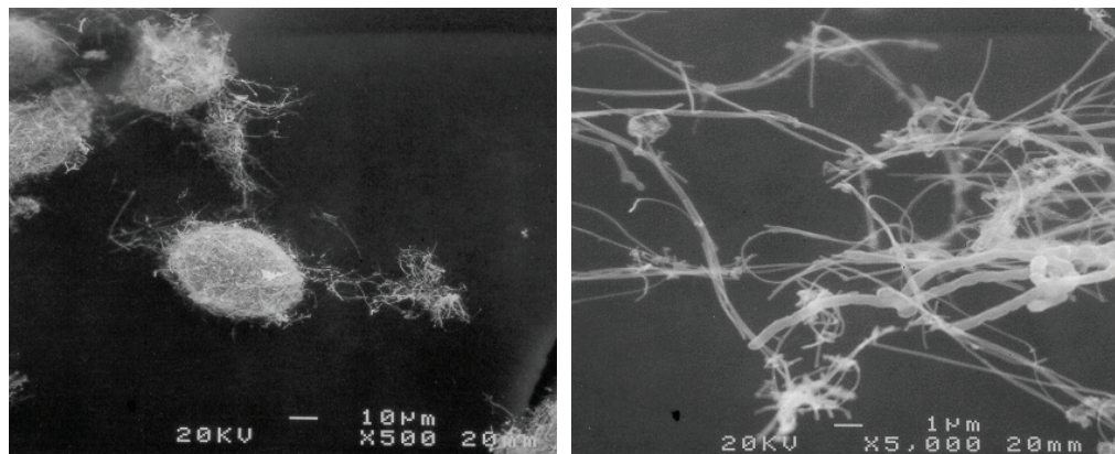
Bulk multi-walled carbon nanotubes observed as an agglomerated “bird’s nest” and as a loose bundle
